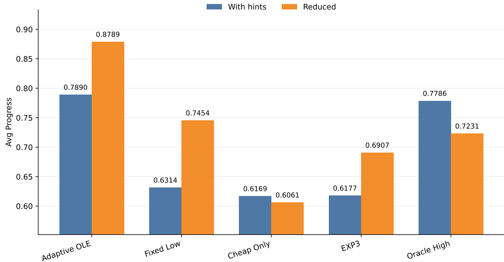
Figure 3: Prompt Ablation: With Hints vs Reduced
